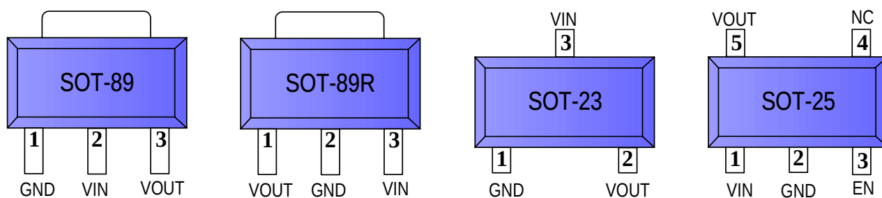
Figure 2 : pin configuration
