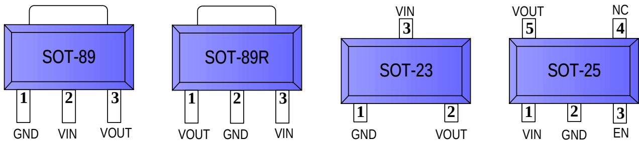
Figure 2 : pin configuration
