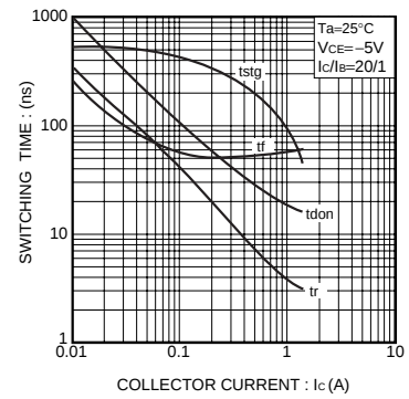
Fig.13 Switching time
