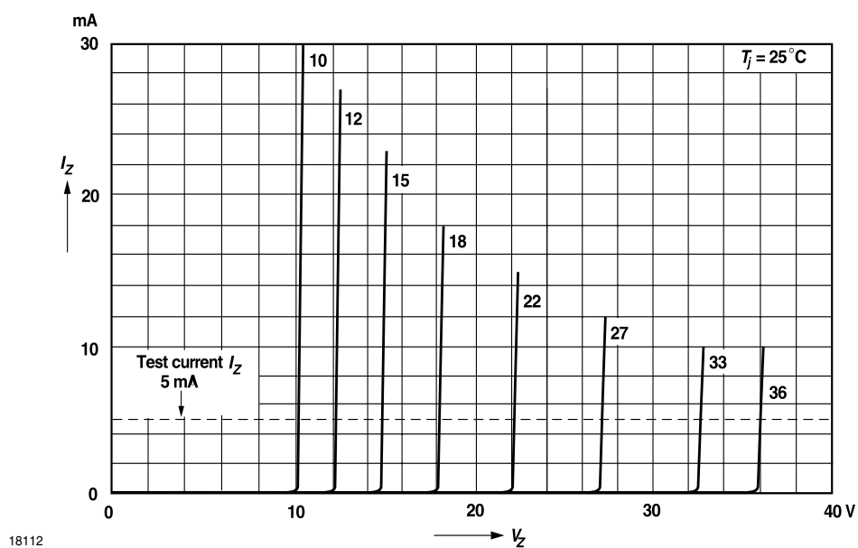
Figure 17. Breakdown Characteristics
