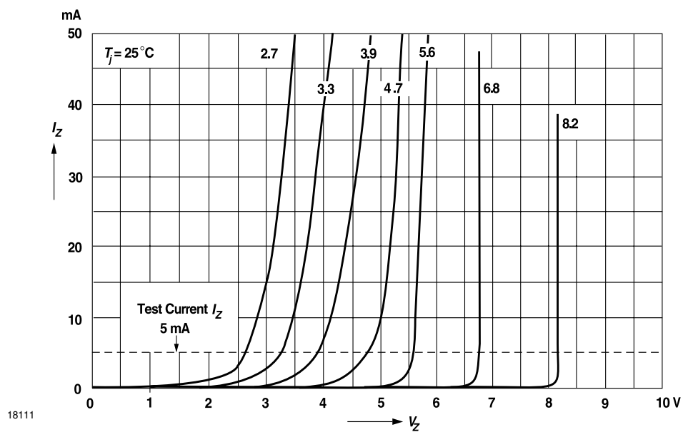
Figure 16. Breakdown Characteristics
