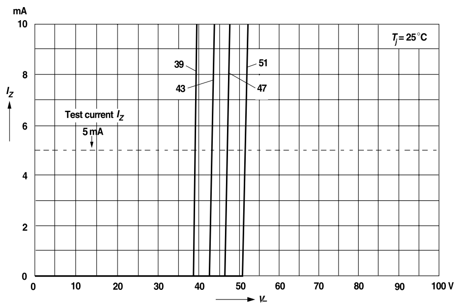
Figure 18. Breakdown Characteristics
