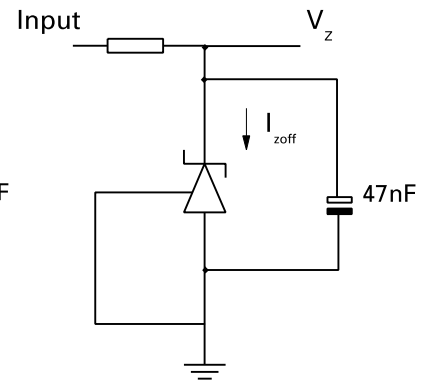
Fig 3 - Test Circuit for Off State current
