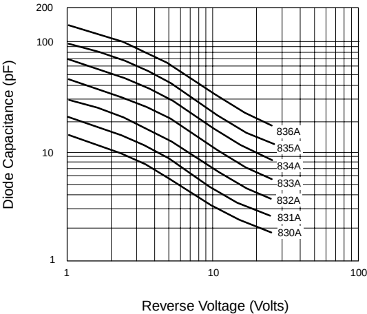
Diode Capacitance
