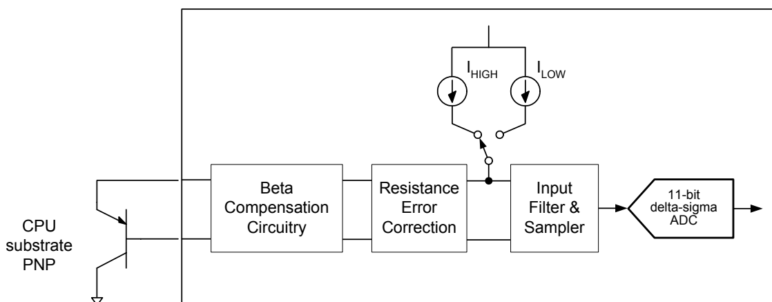
Figure 3.2 Block Diagram of Temperature Monitoring
